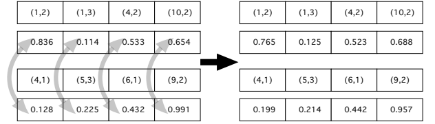
Fig. 2. Coding scheme and crossover operation: an individual is a sparse matrix, which is represented by a list of indices and a list of values.
