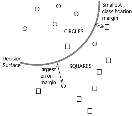
Fig. 1. The fitness of an ensemble has three components: (a) a quantile of the bootstrap estimation of the training error, (b) the largest distance between a misclassified example and the decision surface, and (c) the smallest distance between a correctly classified example and the decision surface.
