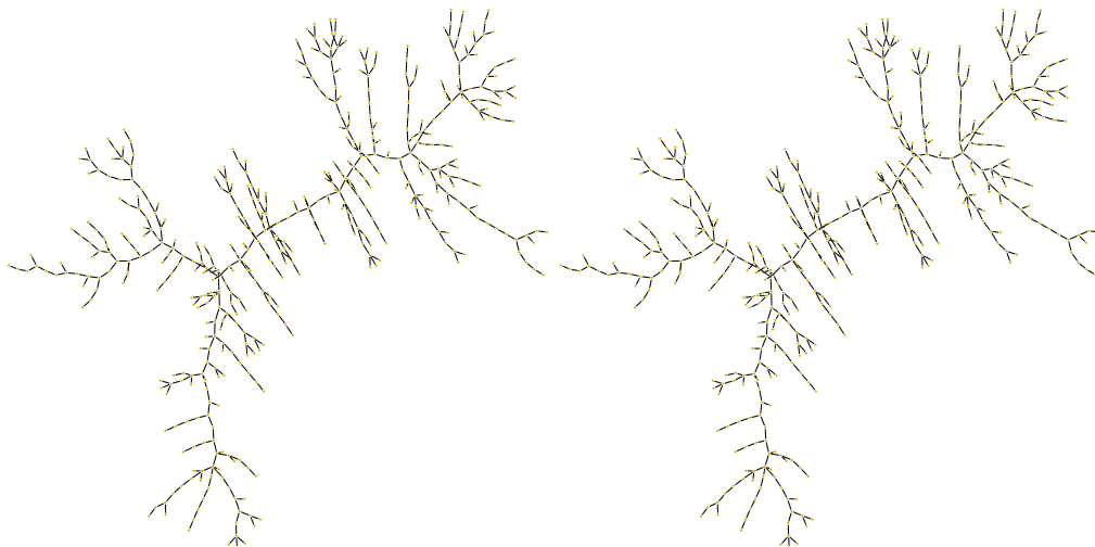
Fig. 8. Comparison of the results obtained by the Binary Pathfinder algorithm (left) and the Fast Pathfinder algorithm (right) on a 500-nodes map generated randomly.
