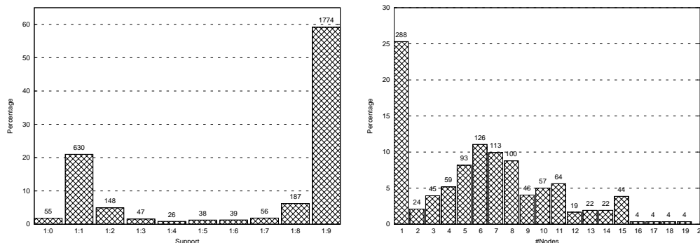
Figure 9: Support and size histograms of the extracted substructures in the leave-one-in experiment
